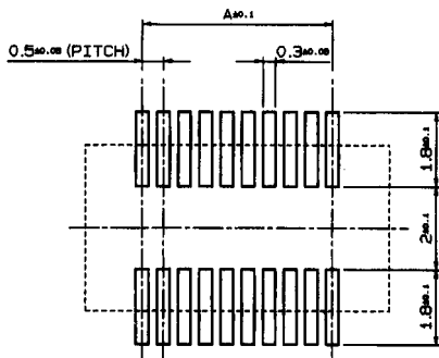
MOUNTING LAYOUT
